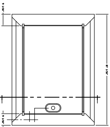
HORIZONTAL SECTION
